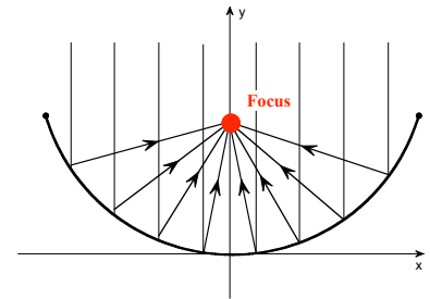
This diagram shows the unique properties of the parabola.
